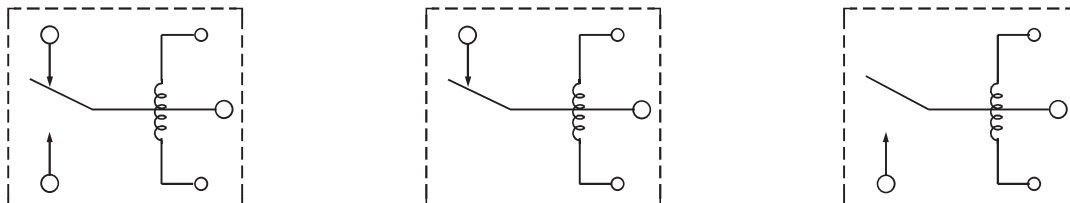
Wiring diagram (bottom view) 接线图 (底视图)
